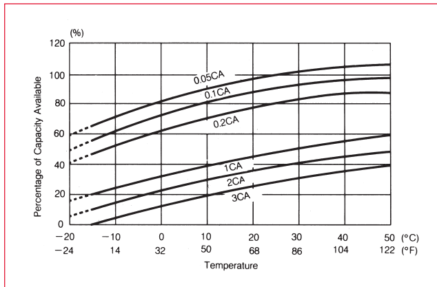
Figure 8. Temperature Effects in Relation to Battery Capacity
