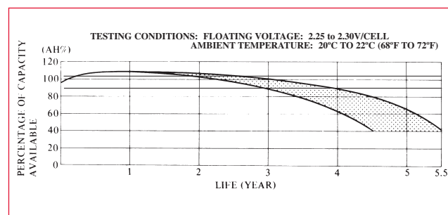
Figure 17. Float Service Life
