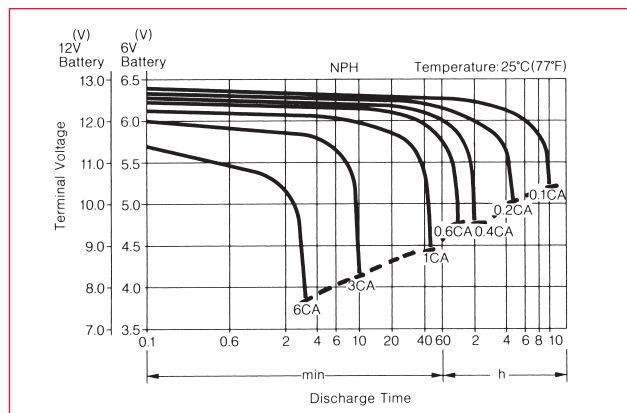
Figure 4. Discharge Characteristic Curves: Genesis NPH Batteries
