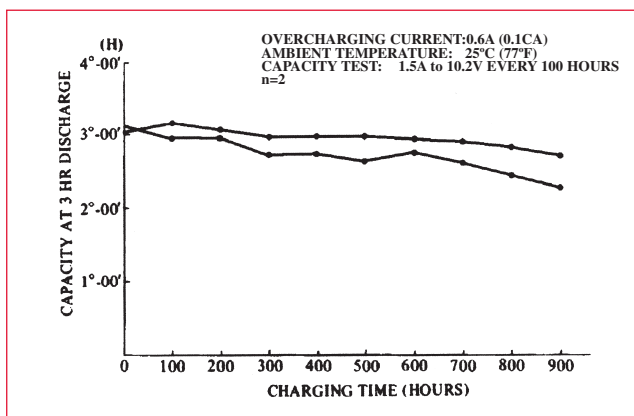
Figure 9. Overcharge Characteristics of NP7-12 Under Continuous Overcharge
